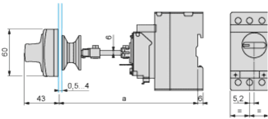
Door cut-out
