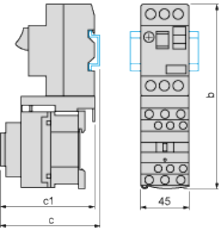
Combination GV2ME + TeSys d contactor
