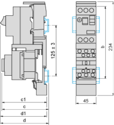
Combination GV2ME + TeSys d contactor
