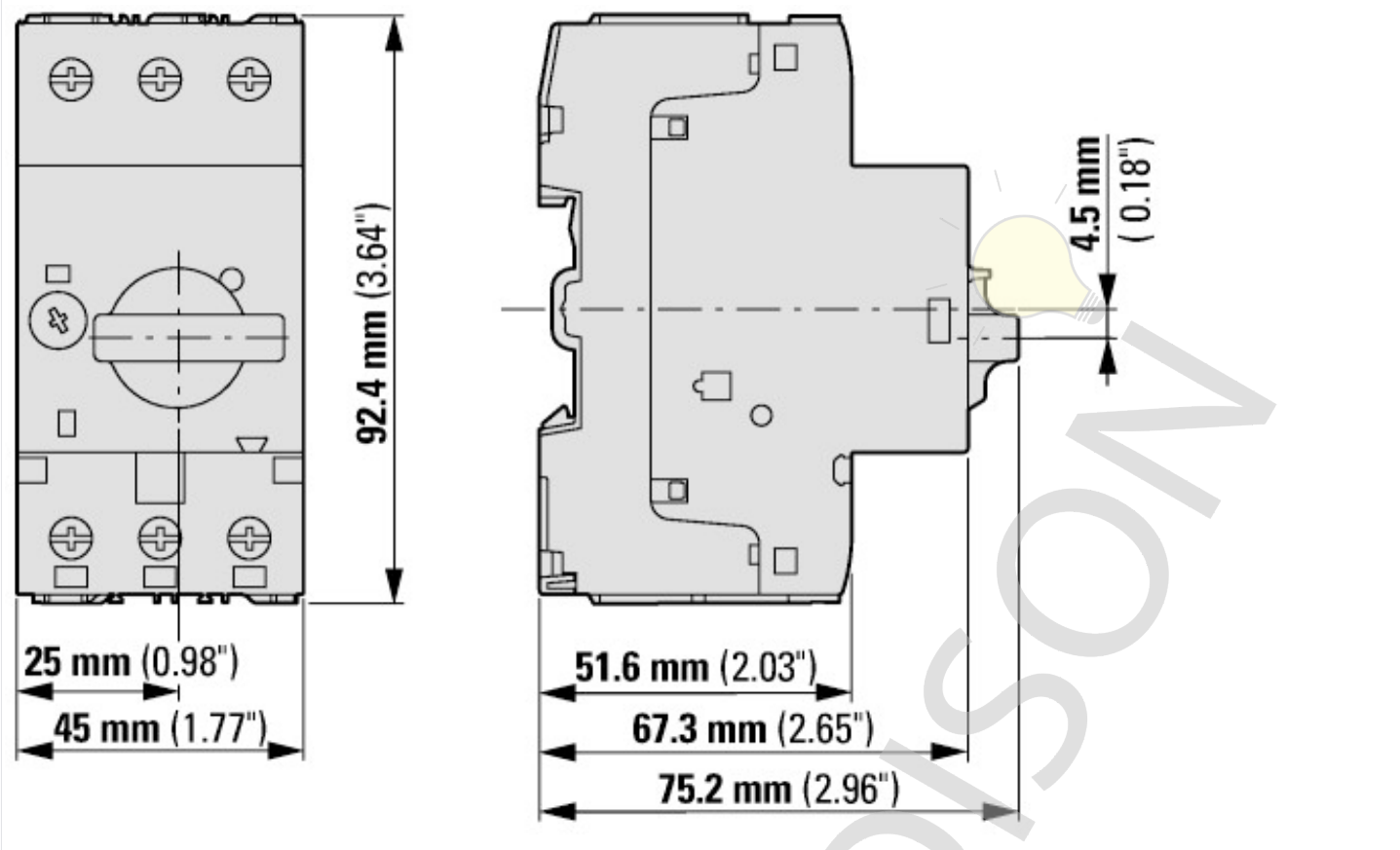
Motor-protective circuit-breaker with standard auxiliary contact PKZM0-...(+NHI-E-...-PKZ0) PKZM0-...-T(+NHI-E-...-PKZ0) PKM0-...(+NHI-E-...-PKZ0)
