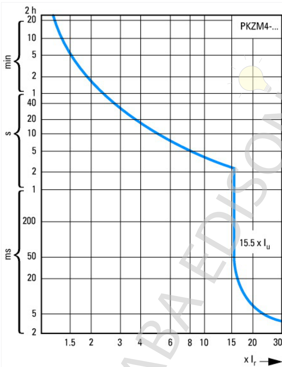
Tripping characteristics motor-protective circuit breaker PKZM4-...
