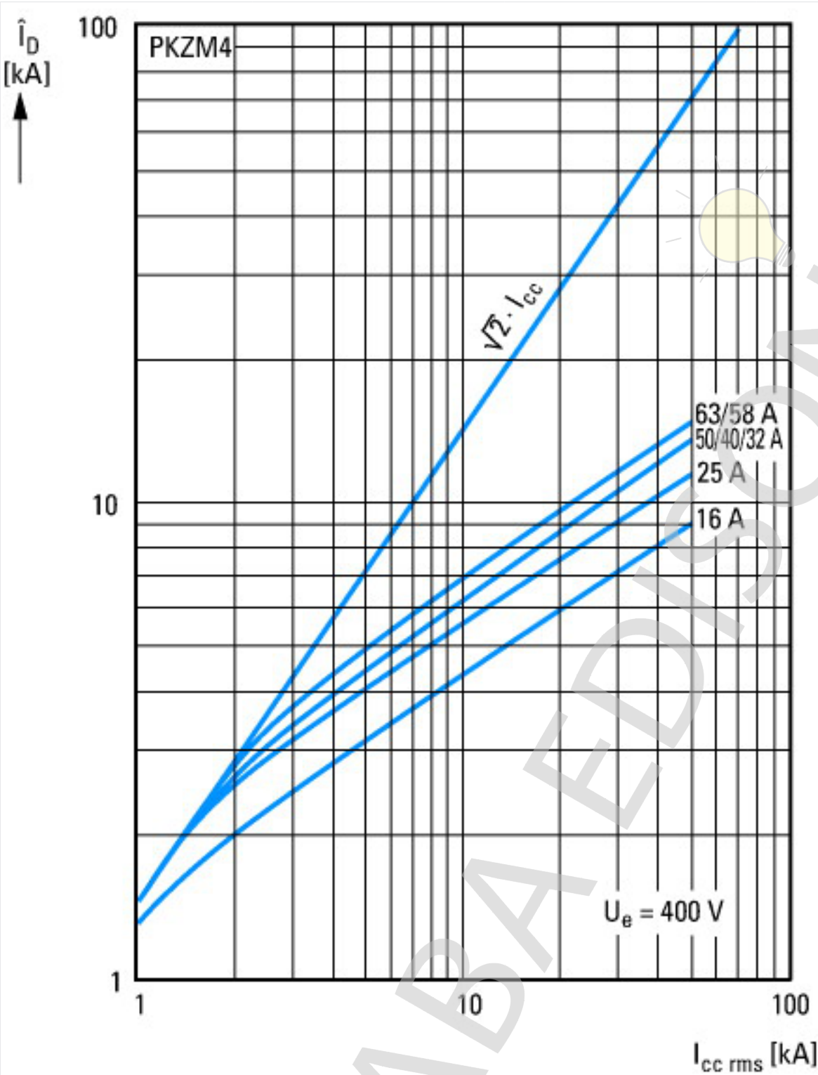
Let-through current
